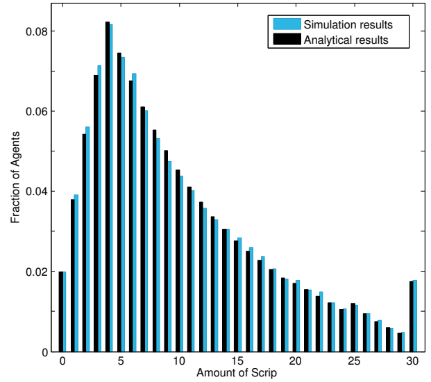
Fig. 1. Distribution of scrip with n = 5 and k_t = 30 for 1000 agents. Dark (black) bars represent the theoretical distribution obtained in Theorem 1, whereas simulation results (after 10,000 iterations) are shown in light (blue).
