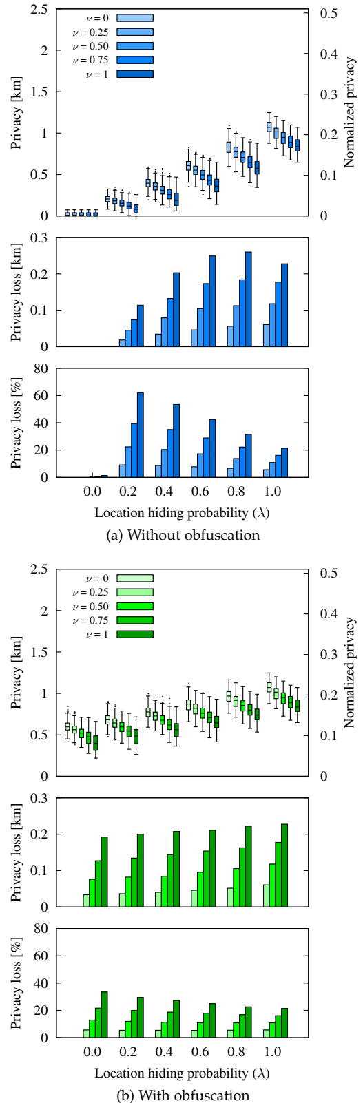
Fig. 5. Privacy (top), absolute privacy loss (middle) and relative privacy loss (bottom) for the limited user set attack with N = 2 users, when users do not report fake co-locations ( \mu = 0 ). The privacy loss is expressed w.r.t. the case where no co-locations are available ( \nu = 0 , \mu = 0 ); the histograms show median values.
